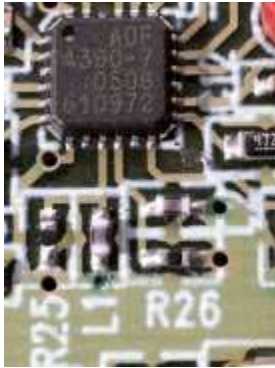
Figure 3. External Inductors and Resistors for ADF4360-7 Tank Circuit
