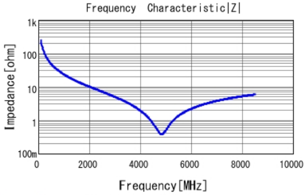
GRM0225C1H6R5CA03 |Z| DCOV, 25degC
