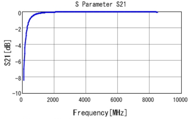
GRM0225C1H6R5CA03 S21 DC0V, 25degC
