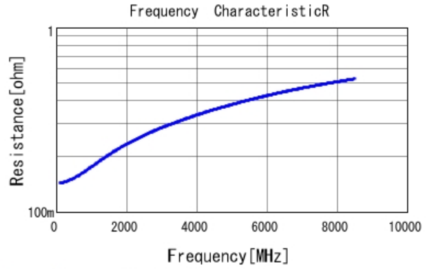
GRM0225C1H6R5CA03 R DCOV, 25degC
