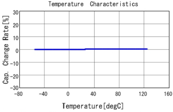
GRM0225C1H6R5CA03 C-Temp. capchange, DC0V, AC1Vrms
