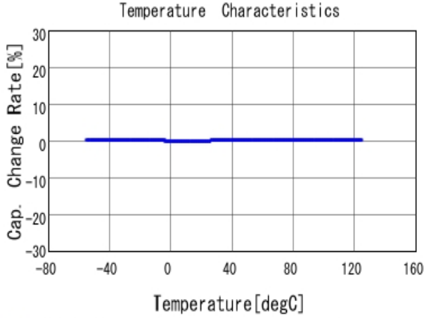
■ GRM0225C1C221GA02 C-Temp. capchange, DCOV, AC1Vrms
