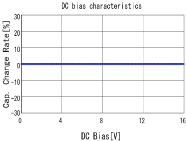
■ GRM0225C1C221GA02 C-DC bias capchange, 25.0degC, AC1V
