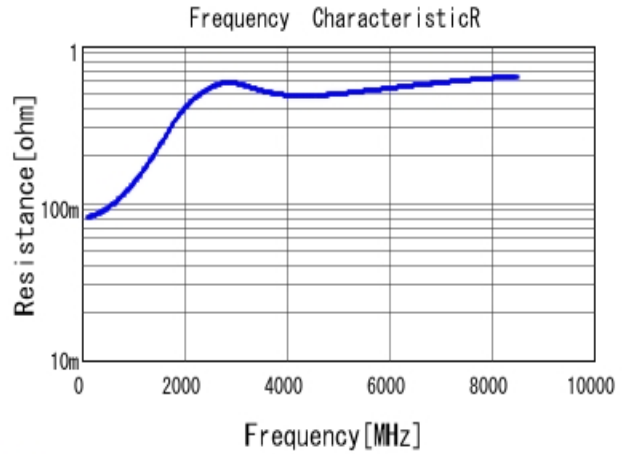
■ GRM0225C1C221GA02 R DC0V, 25degC
