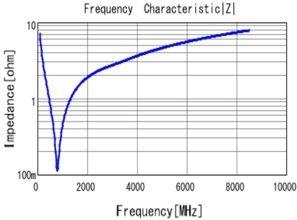
■ GRM0225C1C221GA02 |Z| DC0V, 25degC
