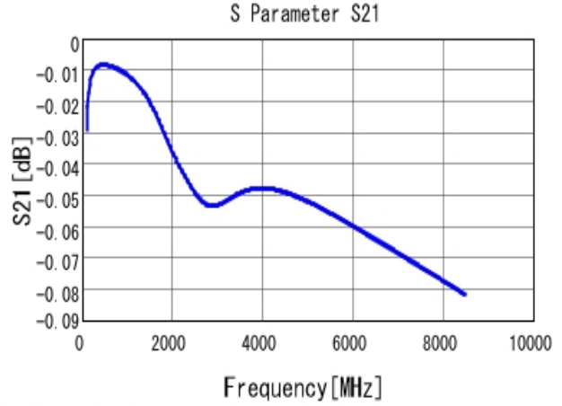
■ GRM0225C1C221GA02 S21 DCOV, 25degC
