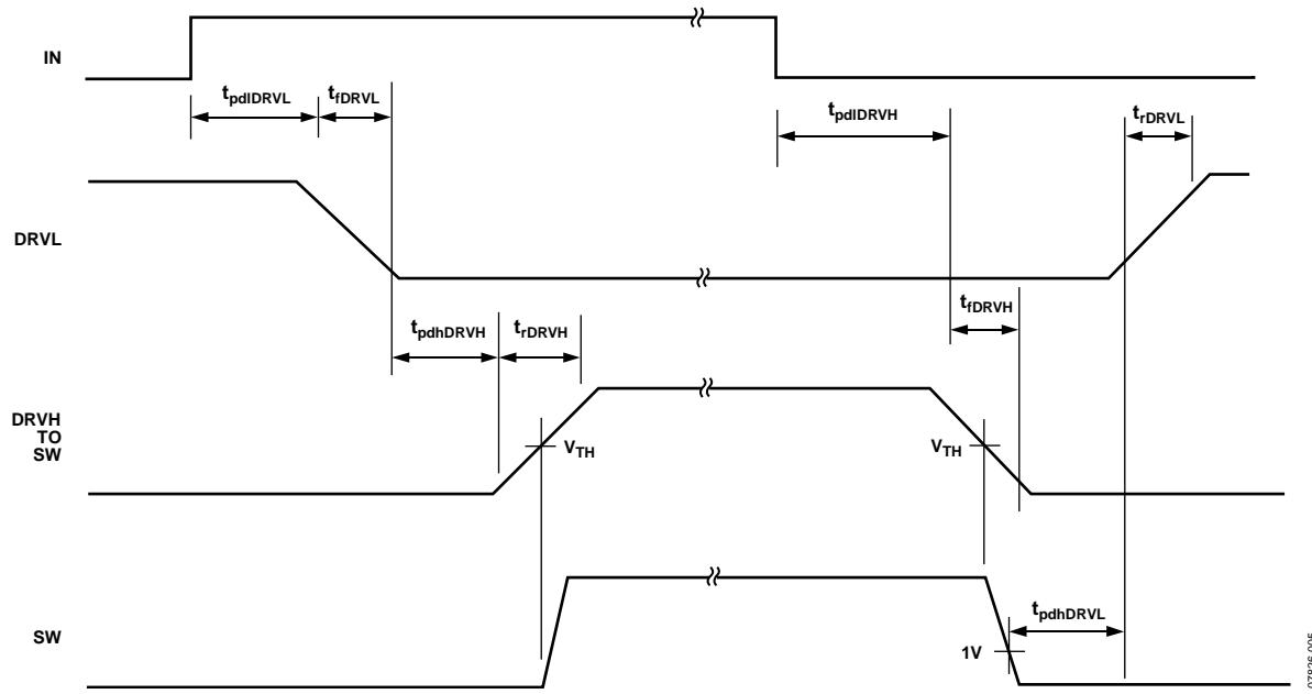
Figure 3. Timing Diagram
