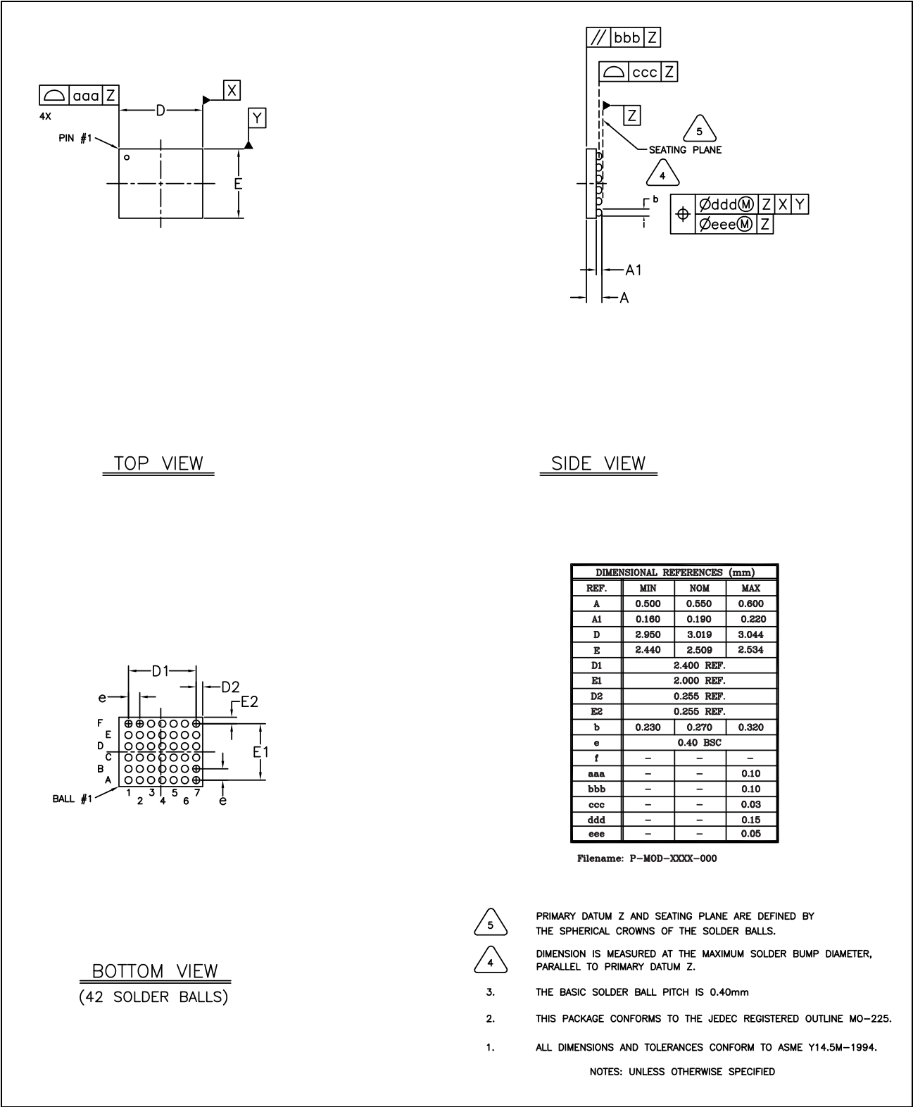
Figure 21: 42-Bump BCM20713A1KUBG Mechanical Drawing
