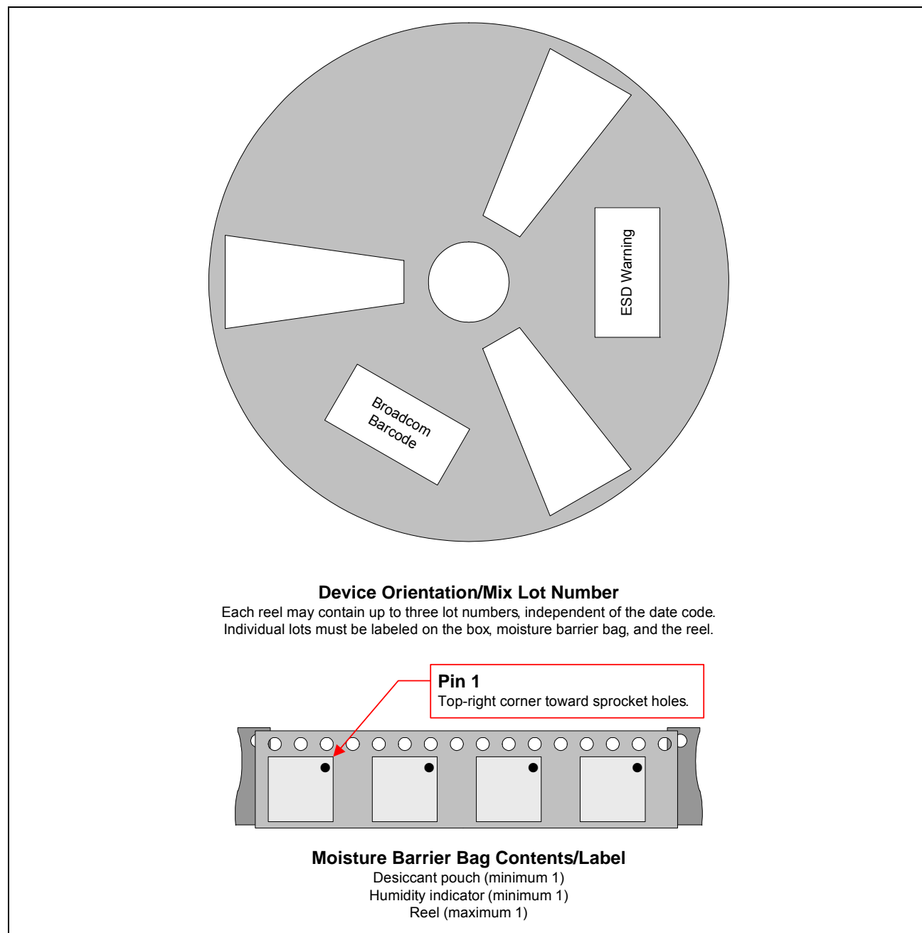
Figure 22: Reel, Labeling, and Packing Specification
