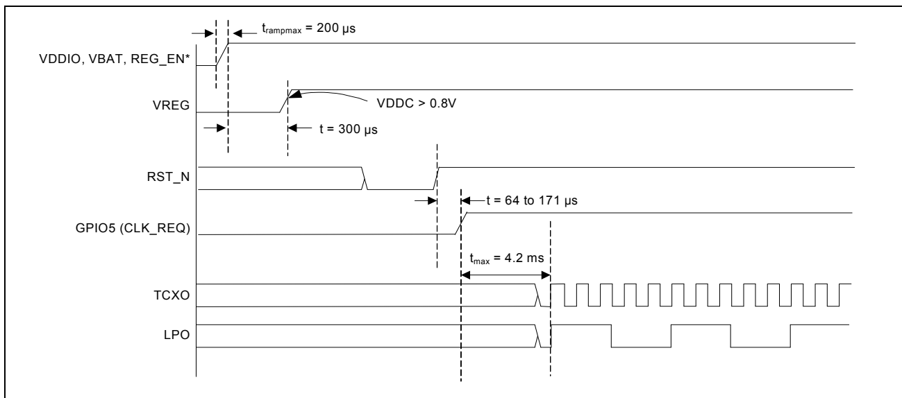
Figure 11: Startup Timing from Power-on Reset
