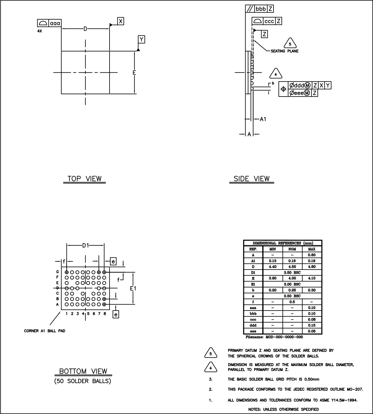
Figure 20: BCM20713A1KUFBXG Mechanical Drawing
