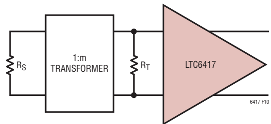
Figure 10. LTC6417 with a Transformer
