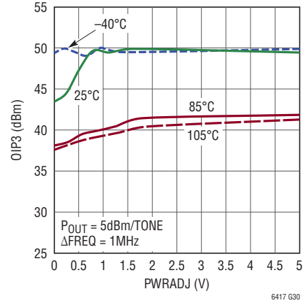
OIP3 at 70MHz vs PWRADJ Over Temperature
