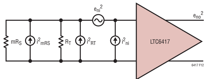
Figure 12. LTC6417 Simplified Noise Model
