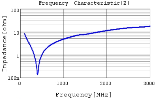
GRM31A5C2J181FW01 |Z| DCOV, 25degC
