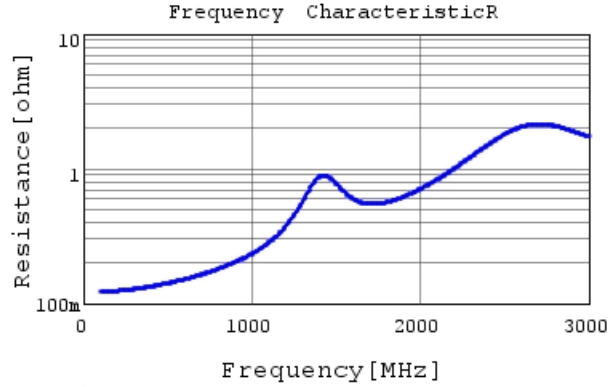
GRM31A5C2J181FW01 R DCOV, 25degC
