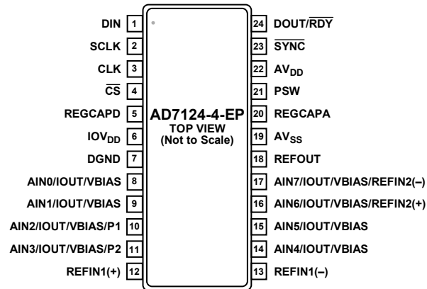
Figure 2. Pin Configuration
