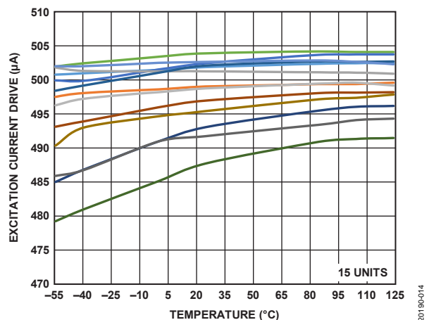
Figure 14. Excitation Current Drift (500 µA)
