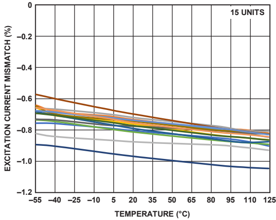
Figure 15. Excitation Current Drift Matching (500 µA)
