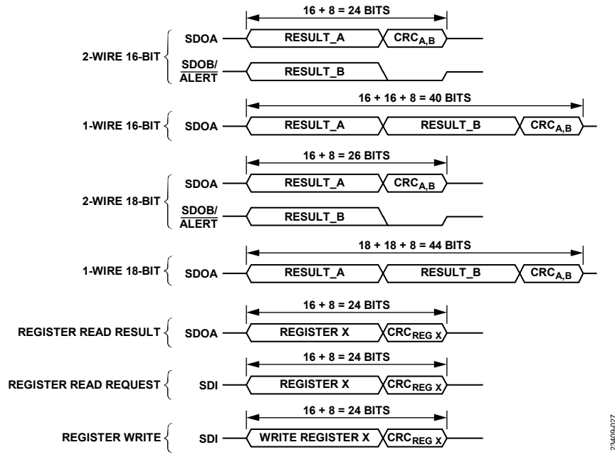
Figure 45. CRC Operation
