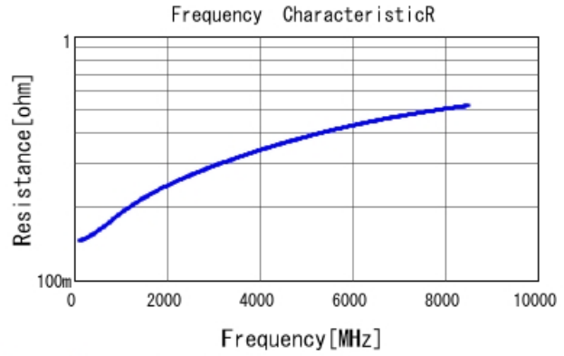
GRM0225C1C6R0CA03 R DCOV, 25degC
