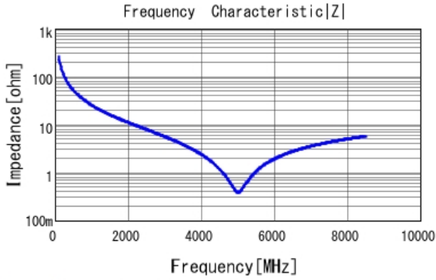
GRM0225C1C6R0CA03 |Z| DCOV, 25degC
