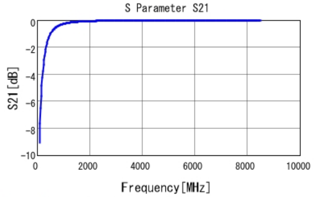
GRM0225C1C6R0CA03 S21 DCOV, 25degC
