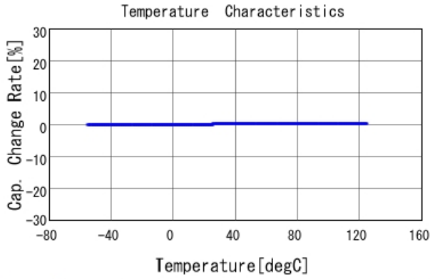
GRM0225C1C6R0CA03 C-Temp. capchange, DCOV, AC1Vrms
