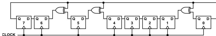
Figure 38. 8-Bit LFSR
