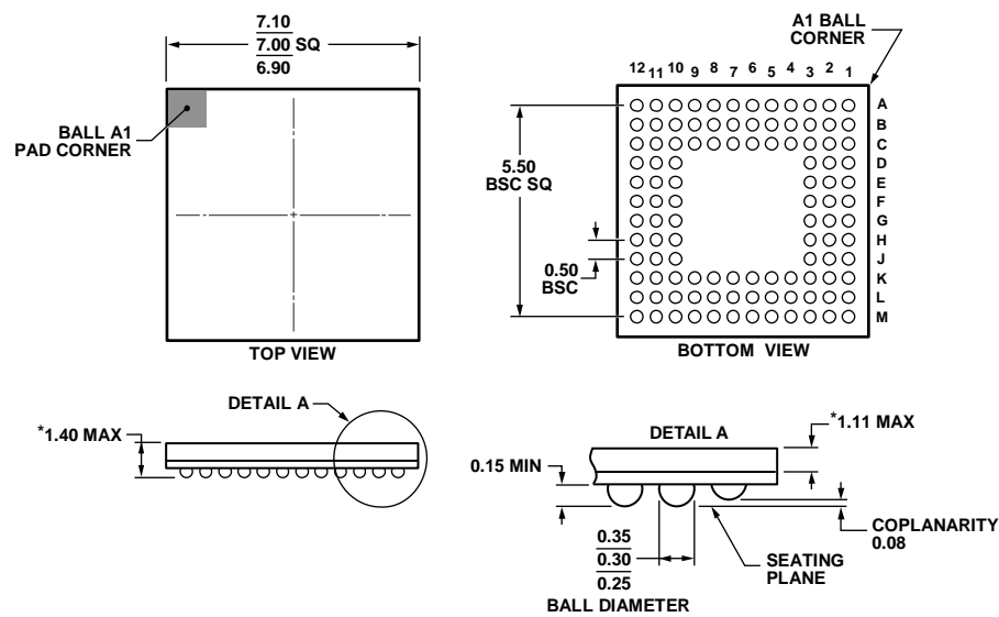
*COMPLIANT WITH JEDEC STANDARDS MO-195-BD WITH EXCEPTION TO PACKAGE HEIGHT AND THICKNESS. Figure 46. 108-Ball Chip Scale Package Ball Grid Array [CSP_BGA] (BC-108-4) Dimensions shown in millimeters
