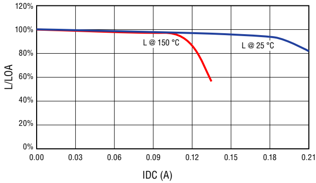
CC453232A-221KL
