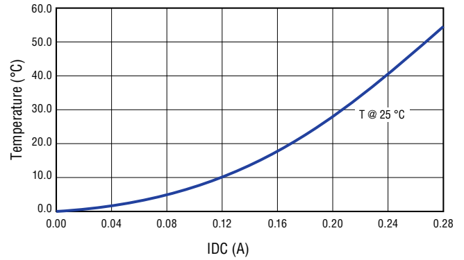
CC453232A-221KL
