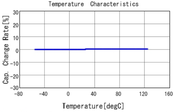
GRM0225C1H7R7CA03 C-Temp. capchange, DCOV, AC1Vrms
