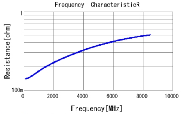
GRM0225C1H7R7CA03 R DCOV, 25degC
