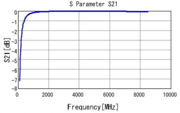
GRM0225C1H7R7CA03 S21 DCOV, 25degC
