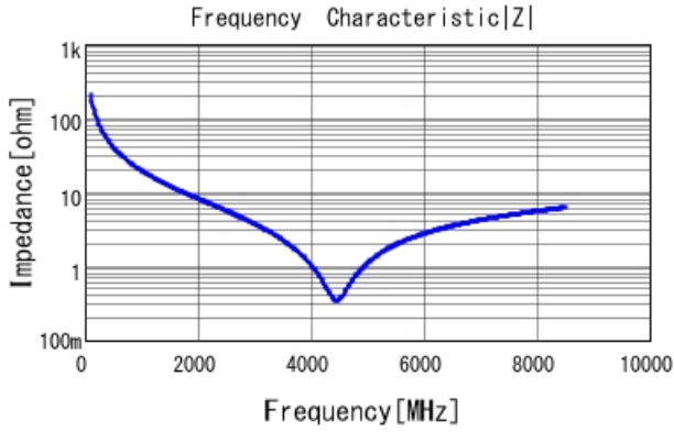
GRM0225C1H7R7CA03 |Z| DCOV, 25degC
