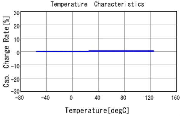
GRM0225C1H6R7BA03 C-Temp. capchange, DCOV, AC1Vrms
