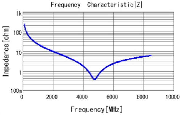
GRM0225C1H6R7BA03 |Z| DCOV, 25degC
