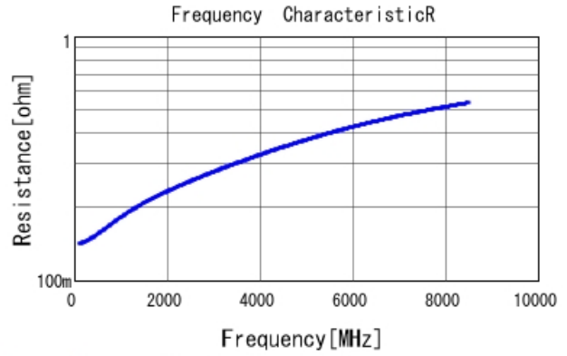
GRM0225C1H6R7BA03 R DCOV, 25degC
