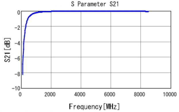
GRM0225C1H6R7BA03 S21 DCOV, 25degC
