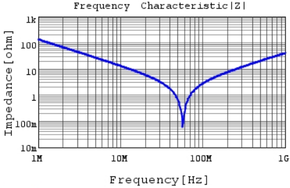
RCE5C2A122J0M1H03A |Z| DCOV, 25degC
