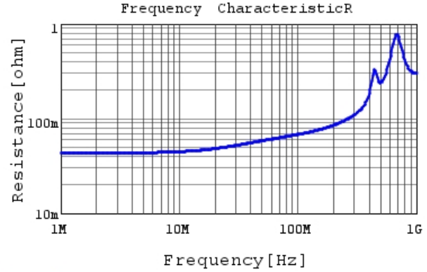
RCE5C2A122J0M1H03A R DCOV, 25degC
