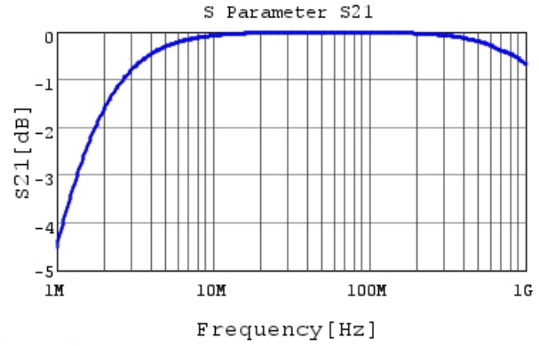
RCE5C2A122J0M1H03A S21 DCOV, 25degC
