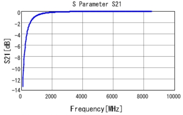
GRM0225C1C3R5CA03 S21 DC0V, 25degC
