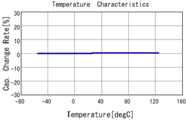
GRM0225C1C3R5CA03 C-Temp. capchange, DC0V, AC1Vrms
