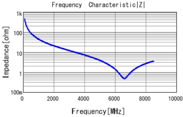
GRM0225C1C3R5CA03 |Z| DCOV, 25degC
