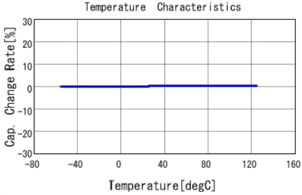
GRM0225C1E130JA03 C-Temp. capchange, DCOV, AC1Vrms
