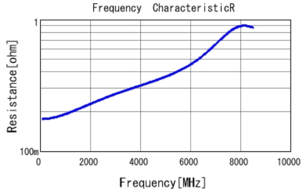
GRM0225C1E130JA03 R DCOV, 25degC
