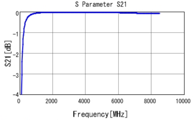
GRM0225C1E130JA03 S21 DCOV, 25degC
