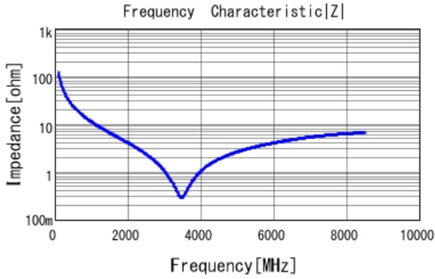
GRM0225C1E130JA03 |Z| DCOV, 25degC
