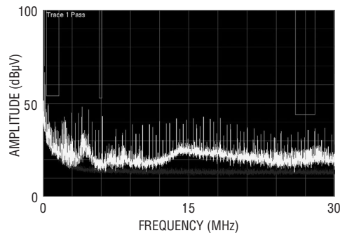
CISPR-25 CONDUCTED EMI MEASUREMENT V IN = 13.5V, I OUT = 8A
