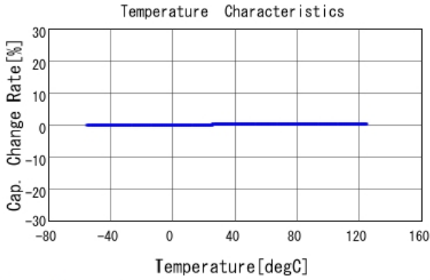
GRM0225C1C1R8CA03 C-Temp. capchange, DCOV, AC1Vrms
