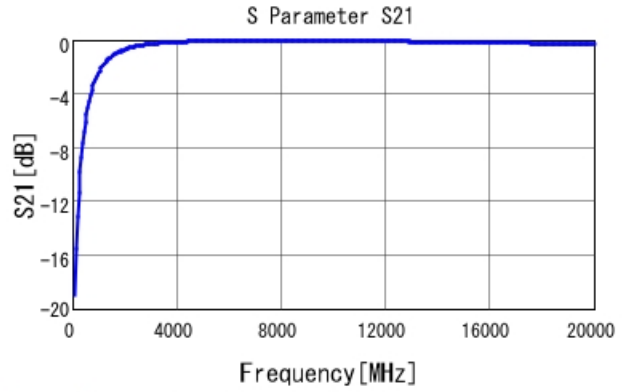
GRM0225C1C1R8CA03 S21 DCOV, 25degC
