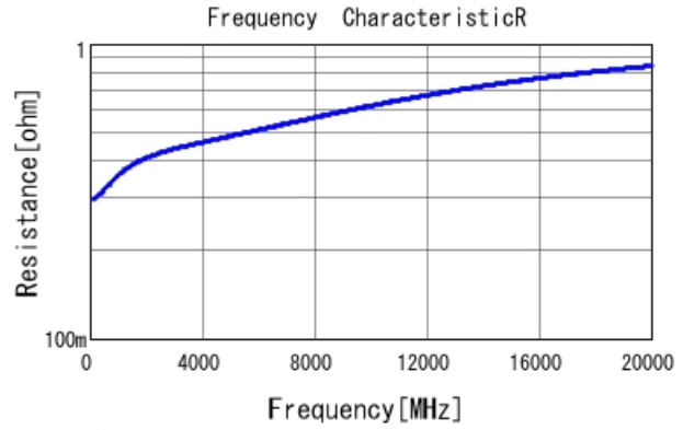
GRM0225C1C1R8CA03 R DCOV, 25degC
