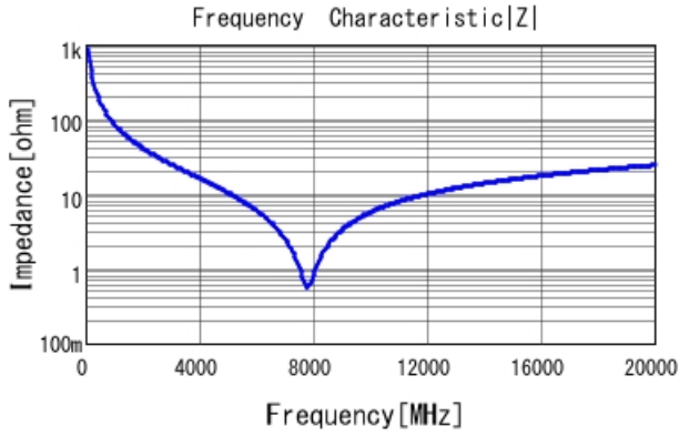
GRM0225C1C1R8CA03 |Z| DCOV, 25degC
