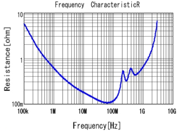
■ GR443QR73D392KW01 R DC0V, 25degC
