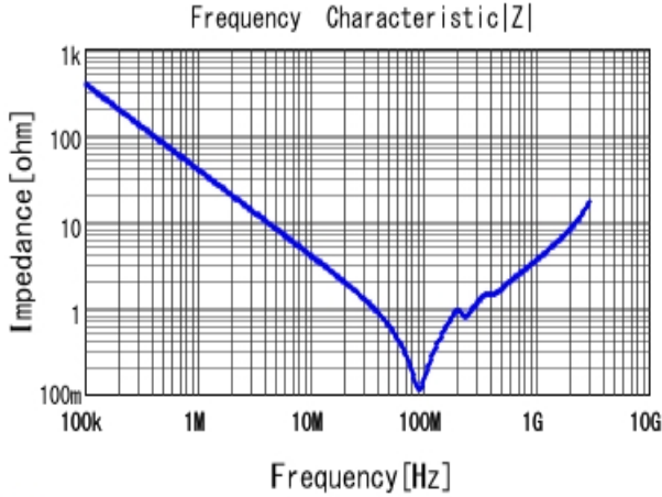
■ GR443QR73D392KW01 |Z| DC0V, 25degC
