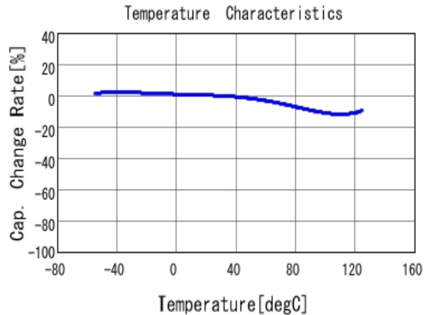
■ GR443QR73D392KW01 C-Temp. capchange, DC0V, AC1Vrms
