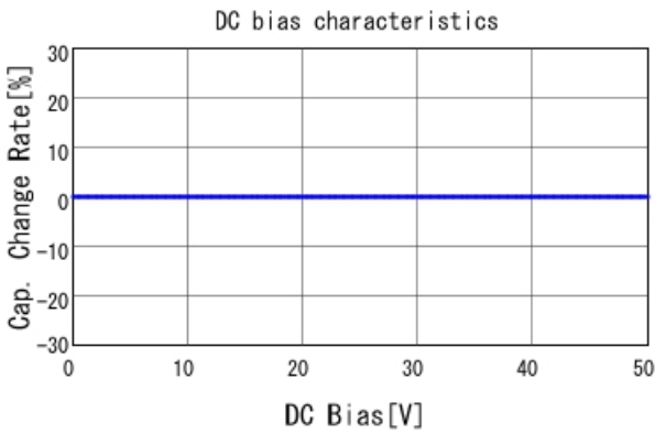
■ GRM0225C1H240JA02 C-DC bias capchange, 25.0degC, AC1V
