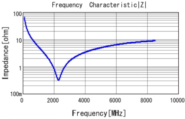
■ GRM0225C1H240JA02 |Z| DCOV, 25degC
