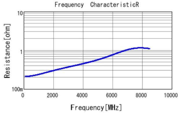
■ GRM0225C1H240JA02 R DCOV, 25degC
