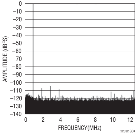
LTC2203: 128K Point FFT, f IN = 1MHz, -1dBFS, PGA = 0
