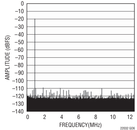
LTC2203: 128K Point FFT, f IN = 1MHz, -20dBFS, PGA = 0
