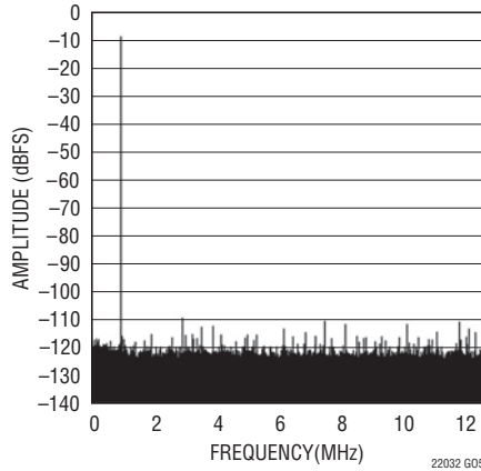
LTC2203: 128K Point FFT, f IN = 1MHz, -10dBFS, PGA = 0
