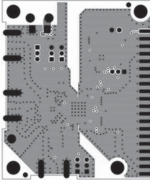
Silkscreen Bottom Side
