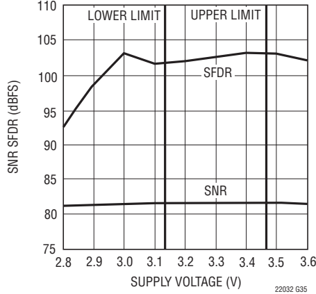
LTC2203: SNR and SFDR vs Supply Voltage ( V_{DD} ), f_{IN} = 5\text{MHz}
