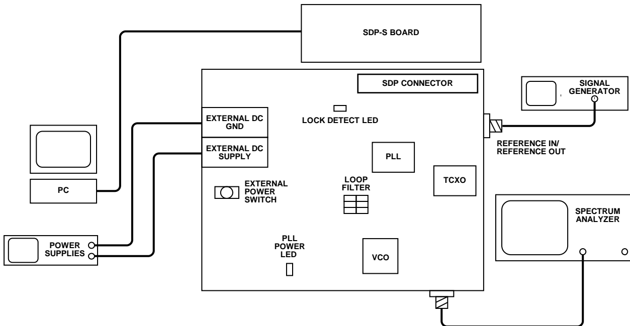
Figure 36. Typical Evaluation Setup
