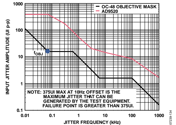
Figure 25. Telcordia GR-253 Jitter Tolerance Plot
