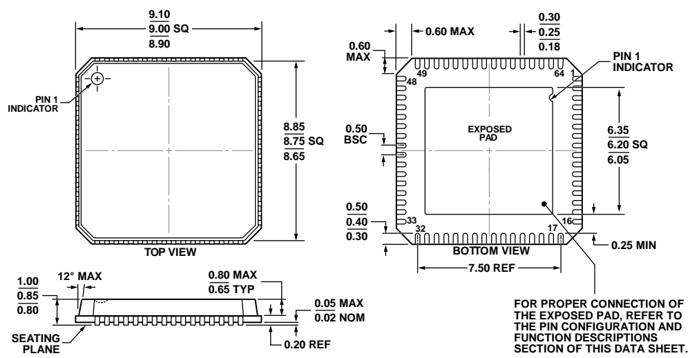
Figure 64. 64-Lead Lead Frame Chip Scale Package [LFCSP_VQ] 9 mm x 9 mm Body, Very Thin Quad CP-64-4 Dimensions shown in millimeters
