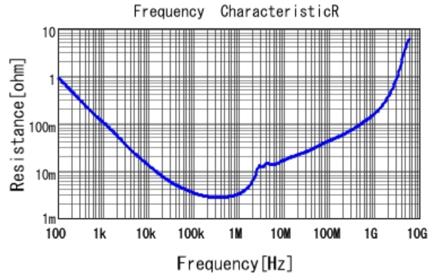
GRT31CC81A106ME01 R DCOV, 25degC
