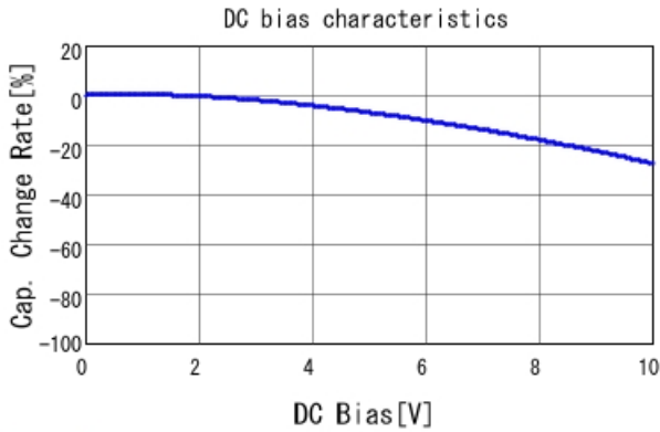
GRT31CC81A106ME01 C-DC bias capchange, 25.0degC, A
