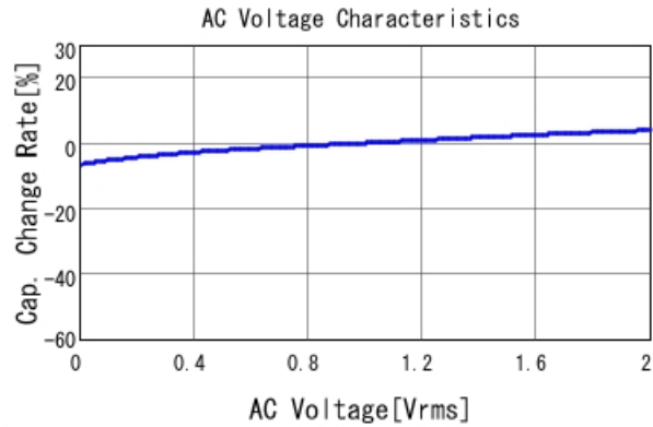
GRT31CC81A106ME01 C-AC Voltage capchange, DCOV, 25
