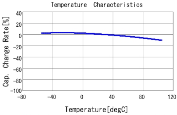
GRT31CC81A106ME01 C-Temp. capchange, DC0.0V, AC1.C
