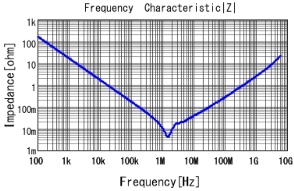
GRT31CC81A106ME01 |Z| DCOV, 25degC
