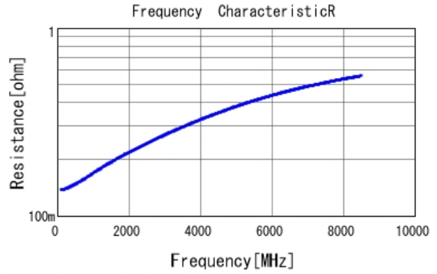
GRM0225C1H8R0WA03 R DCOV, 25degC
