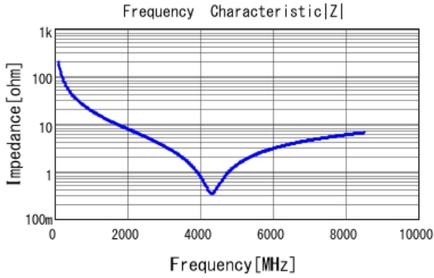
GRM0225C1H8R0WA03 |Z| DCOV, 25degC
