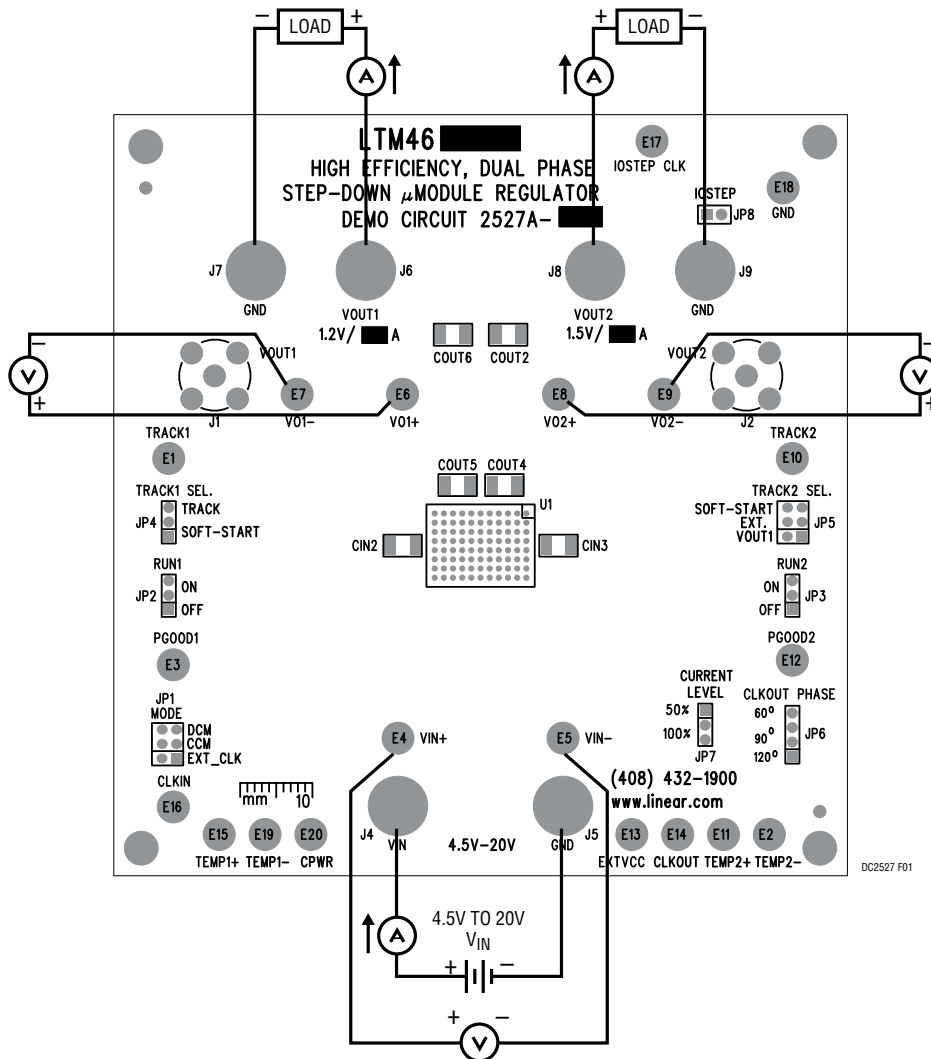
Figure 1. Measurement Setup of DC2527A
