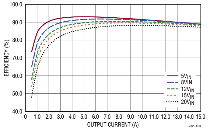
Figure 3. Measured Efficiency of Channel 2 at V_{OUT1} = 1.5V , f_{SW} = 350kHz , CCM
