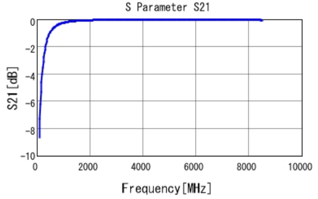
GRM0225C1C6R3WA03 S21 DCOV, 25degC
