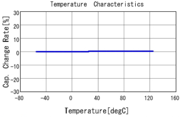
GRM0225C1C6R3WA03 C-Temp. capchange, DCOV, AC1Vrms
