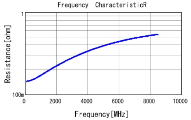
GRM0225C1C6R3WA03 R DCOV, 25degC
