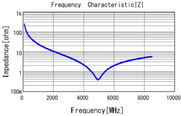
GRM0225C1C6R3WA03 |Z| DCOV, 25degC
