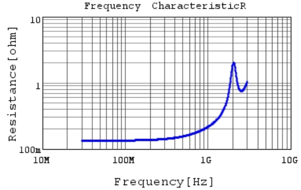
RCE5C1H470J0K1H03B R DC0V, 25degC
