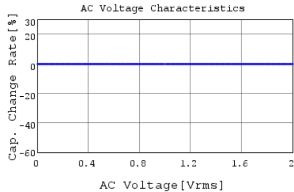
RCE5C1H470J0K1H03B C-AC Voltage capchange, I
