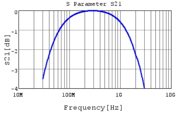
RCE5C1H470J0K1H03B S21 DC0V, 25degC
