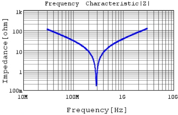
RCE5C1H470J0K1H03B |Z| DC0V, 25degC
