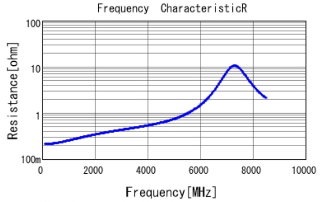
GRM1555C1E5R6DA01 R DCOV, 25degC
