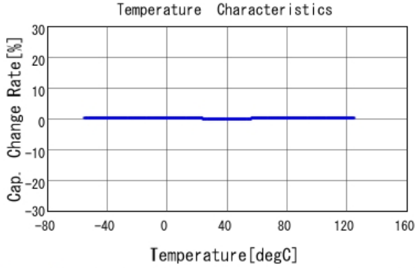
GRM1555C1E5R6DA01 C-Temp. capchange, DCOV, AC1Vrms
