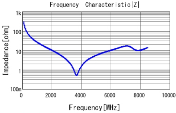
GRM1555C1E5R6DA01 |Z| DCOV, 25degC
