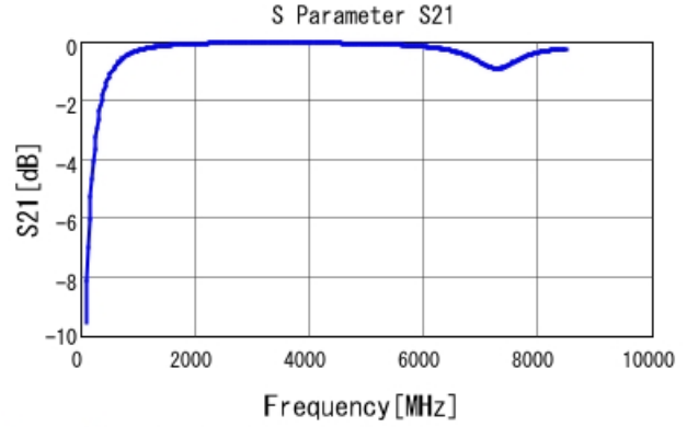
GRM1555C1E5R6DA01 S21 DCOV, 25degC
