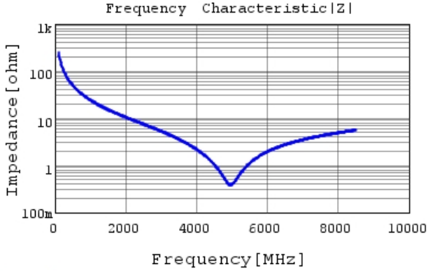
GRM0225C1H6R3DA03 |Z| DCOV, 25degC
