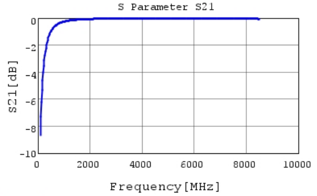
GRM0225C1H6R3DA03 S21 DCOV, 25degC
