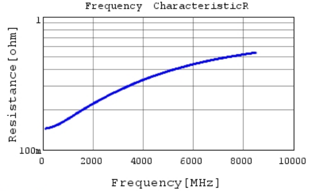
GRM0225C1H6R3DA03 R DCOV, 25degC
