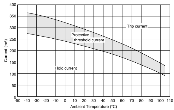
PTGL5SAS100K4B51B0
