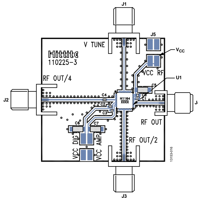
Figure 16. 110225-3 Evaluation PCB
