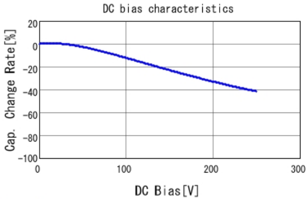
GR355DD72E474KW01 C-DC bias capchange, 25.0degC, A
