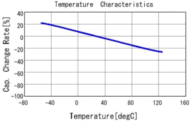
GR355DD72E474KW01 C-Temp. capchange, DCOV, AC1Vrms
