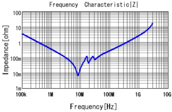
GR355DD72E474KW01 |Z| DCOV, 25degC
