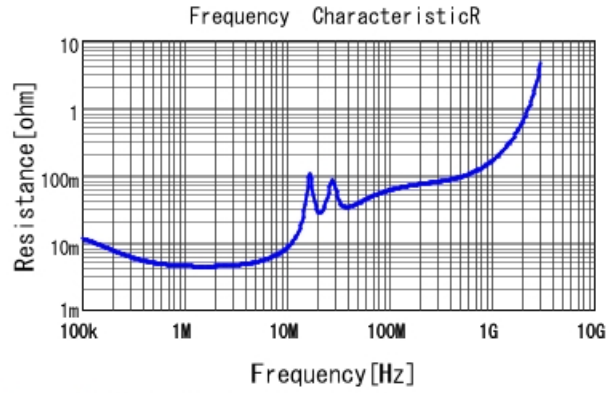
GR355DD72E474KW01 R DCOV, 25degC
