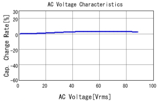
GR355DD72E474KW01 C-AC Voltage capchange, DCOV, 25
