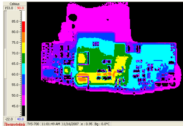
Figure 11. Temp Data (48Vin, 12Aout, 25°C, 200LFM airflow – back)
