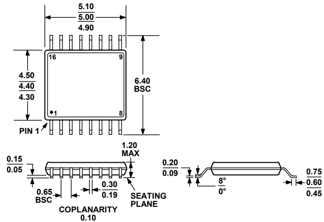
Figure 40. 16-Lead Thin Shrink Small Outline Package [TSSOP] (RU-16)
