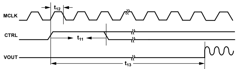
Figure 5. CTRL Timing
