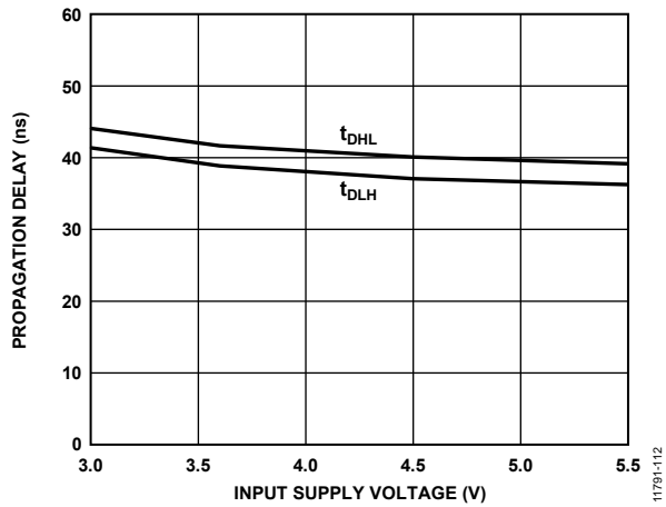
Figure 12. Typical Propagation Delay vs. Input Supply Voltage; V_{DDA}, V_{DDB} = 12V
