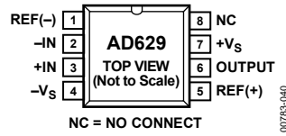
Figure 6. Pin Configuration
