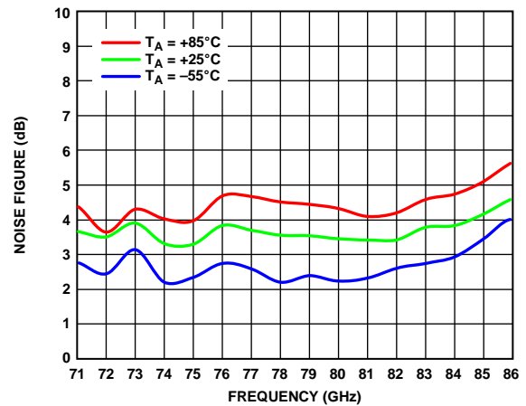
Figure 11. Noise Figure vs. Frequency over Temperature, V_{Dk} = 3\text{ V} , I_{Dk} = 50\text{ mA}
