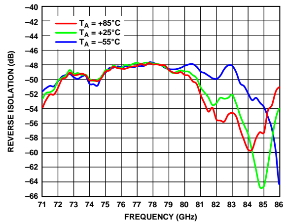
Figure 13. Reverse Isolation vs. Frequency over Temperature, V_{Dk} = 3\text{ V} , I_{Dk} = 57\text{ mA}
