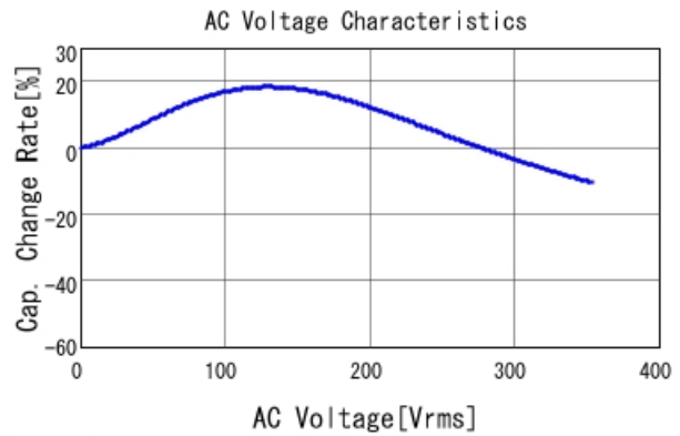
GRJ55DR73A683KWJ1 C-AC Voltage capchange, DCOV, 25
