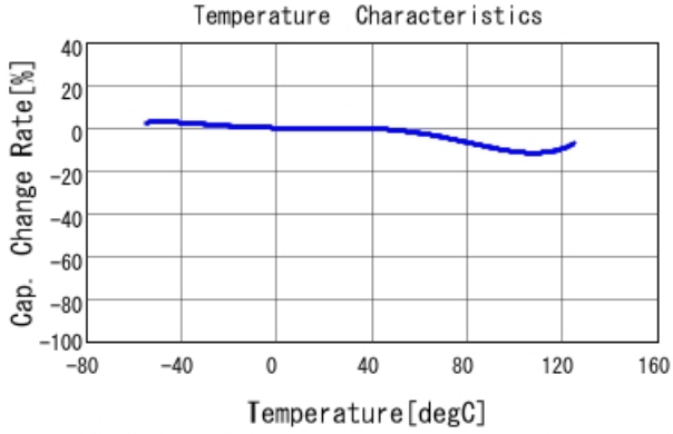
GRJ55DR73A683KWJ1 C-Temp. capchange, DCOV, AC1Vrms
