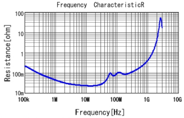
GRJ55DR73A683KWJ1 R DCOV, 25degC
