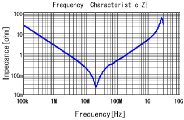
GRJ55DR73A683KWJ1 |Z| DCOV, 25degC
