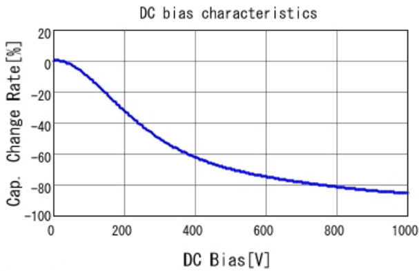
GRJ55DR73A683KWJ1 C-DC bias capchange, 25.0degC, A
