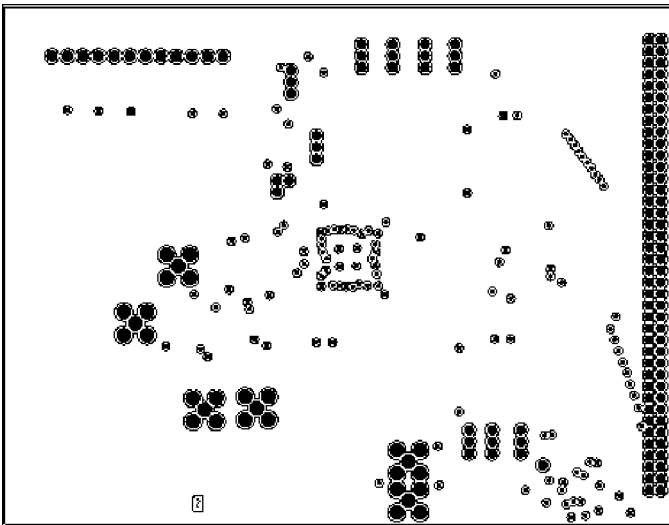
Figure 16. Ground Plane
