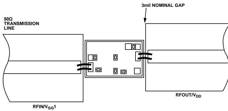
Figure 41. Assembly Diagram
