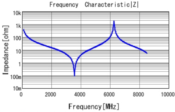
GQM22M5C2H4R0CB01 |Z| DCOV, 25degC
