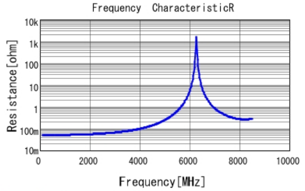
GQM22M5C2H4R0CB01 R DCOV, 25degC
