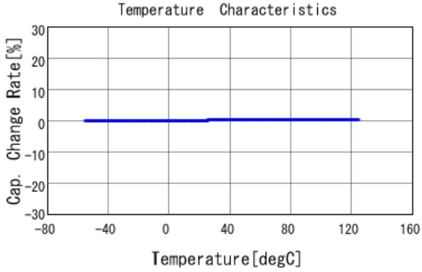
GQM22M5C2H4R0CB01 C-Temp. capchange, DC0V, AC1Vrms
