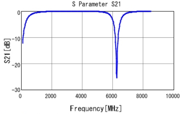
GQM22M5C2H4R0CB01 S21 DC0V, 25degC
