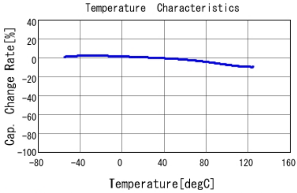
GRM31MR72A474MA35 C-Temp. capchange, DC0.0V, AC1.C
