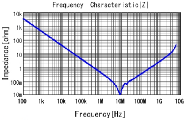
GRM31MR72A474MA35 |Z| DCOV, 25degC
