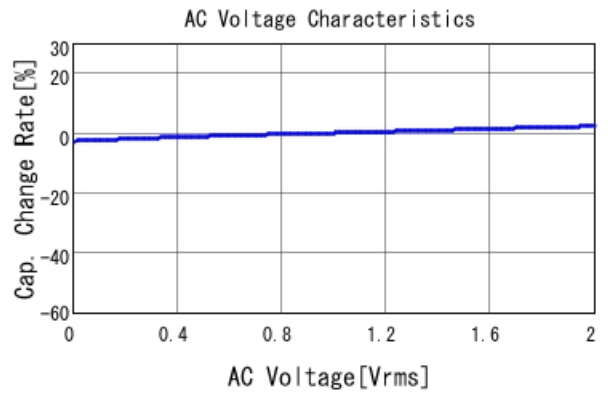
GRM31MR72A474MA35 C-AC Voltage capchange, DCOV, 25
