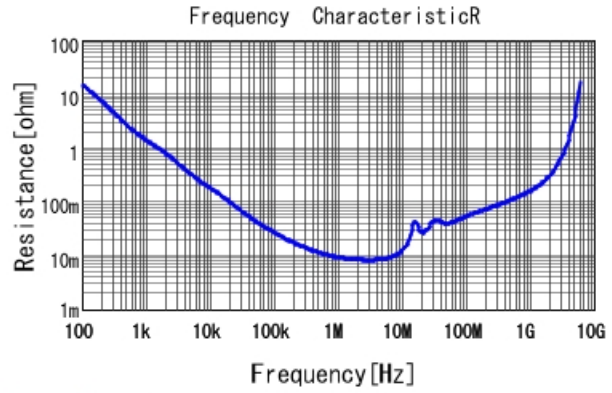
GRM31MR72A474MA35 R DCOV, 25degC
