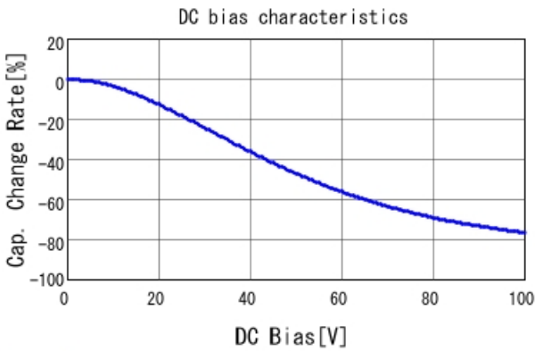
GRM31MR72A474MA35 C-DC bias capchange, 25.0degC, A
