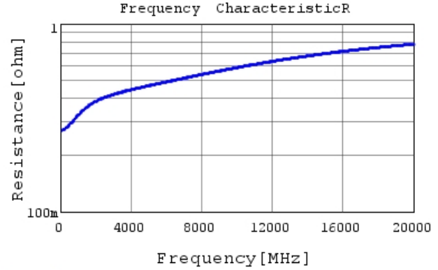
GRM0225C1H2R0WA03 R DCOV, 25degC
