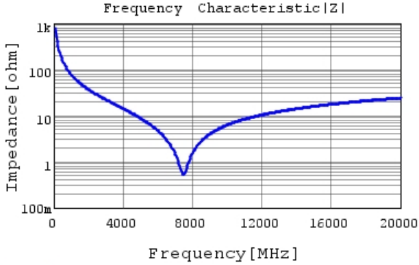
GRM0225C1H2R0WA03 |Z| DCOV, 25degC
