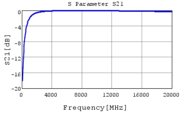
GRM0225C1H2R0WA03 S21 DCOV, 25degC
