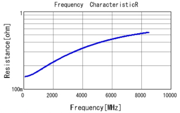
GRM0225C1C6R3BA03 R DCOV, 25degC
