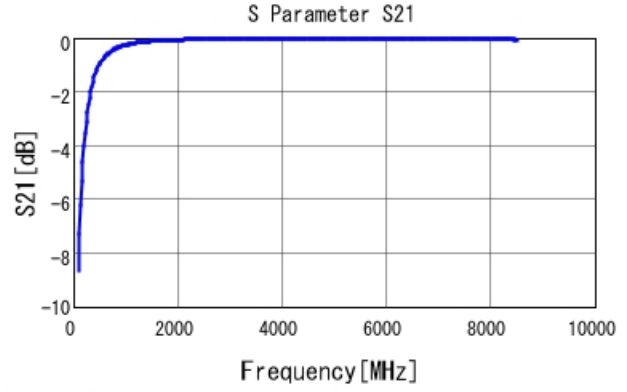
GRM0225C1C6R3BA03 S21 DC0V, 25degC
