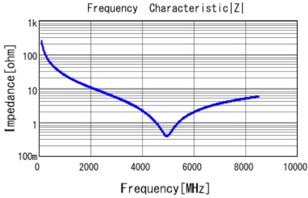
GRM0225C1C6R3BA03 |Z| DCOV, 25degC
