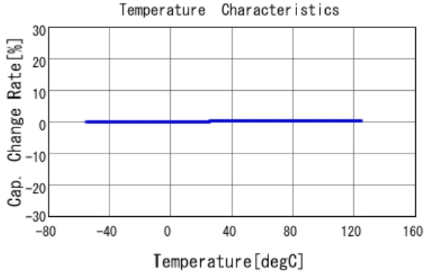
GRM0225C1C6R3BA03 C-Temp. capchange, DC0V, AC1Vrms
