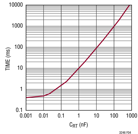
Figure 4. Reset Timeout Period vs C_{\text{RT}} Capacitance
