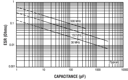
ESR VS. CAPACITANCE ATC SERIES 700, CASE C
