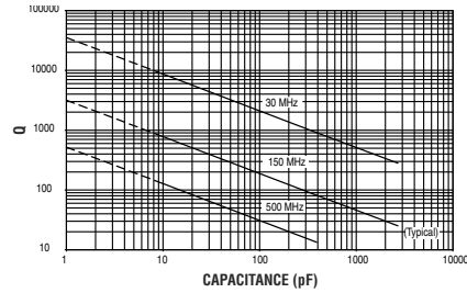
Q VS. CAPACITANCE ATC SERIES 700, CASE C
