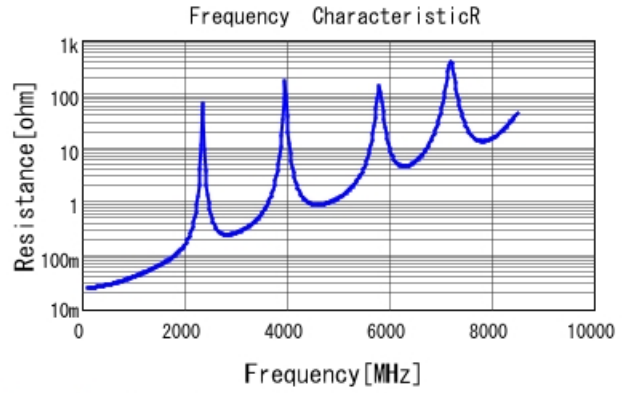
GQM22M5C2H470JB01 R DCOV, 25degC
