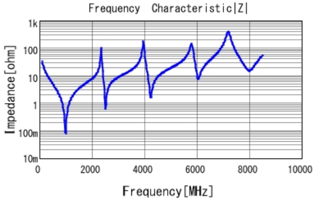
GQM22M5C2H470JB01 |Z| DCOV, 25degC
