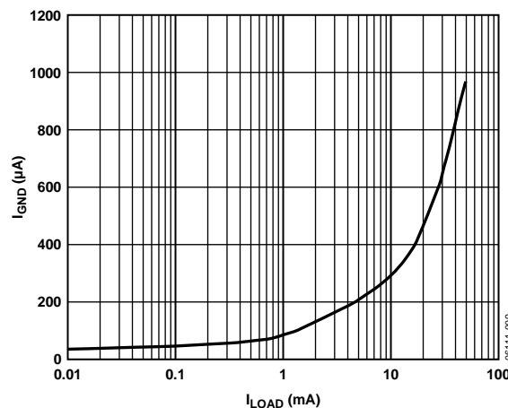
Figure 9. Ground Current vs. Load Current
